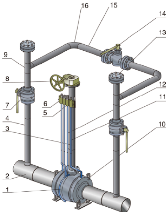
COMPLETE BY-PASS SYSTEM
