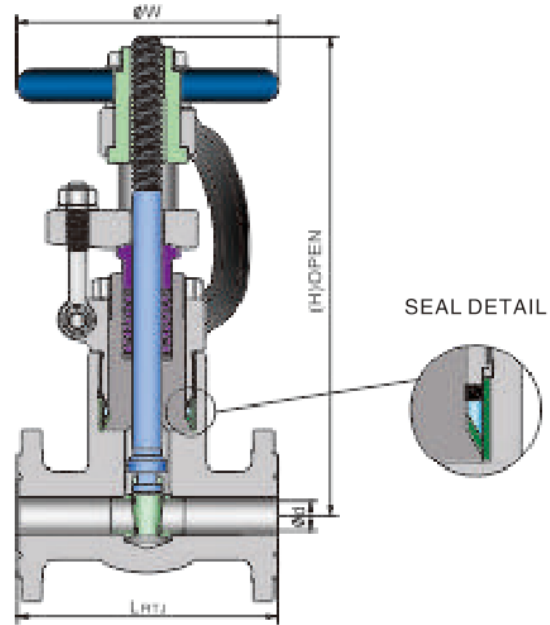
RTJ PRESSURE SEAL BONNET 1500,2500LB
