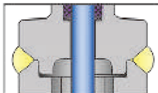
2.Welded Bonnet
