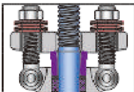
1.Live-loading
