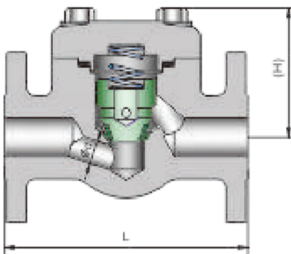
PISTON TYPE CHECK VALVE
