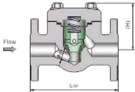
PISTON TYPE, FLANGED BOLTED BONNET 150~1500LB
